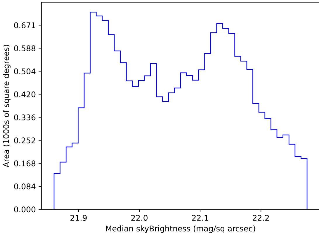
internal_u_expt45_nscale1.5v3.4_10yrs WFD g band: Median skyBrightness
