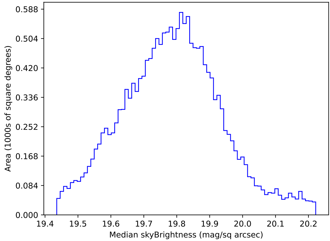
internal_u_expt45_nscale1.5v3.4_10yrs WFD all bands: Median skyBrightness
