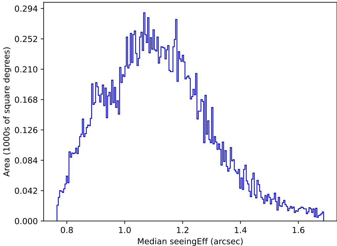
internal_u_expt45_nscale1.5v3.4_10yrs Yr 1 u band: Median seeingEff
