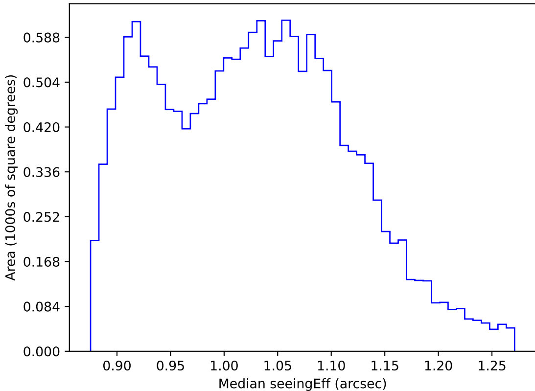
internal_u_expt45_nscale1.5v3.4_10yrs WFD r band: Median seeingEff
