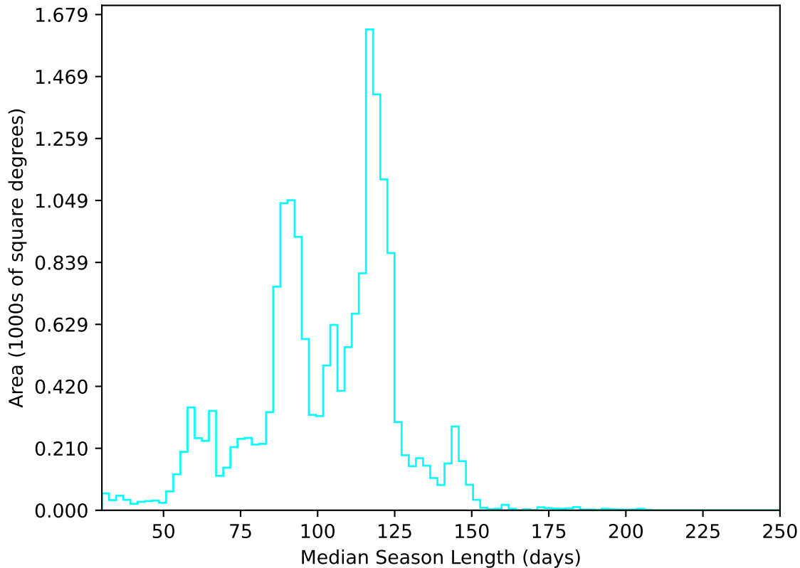
internal_u_expt45_nscale1.5v3.4_10yrs WFD u band: Median Season Length
