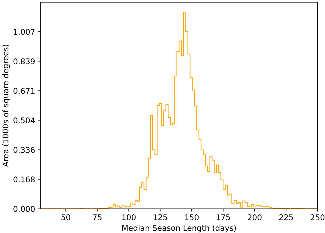
internal_u_expt45_nscale1.5v3.4_10yrs WFD r band: Median Season Length
