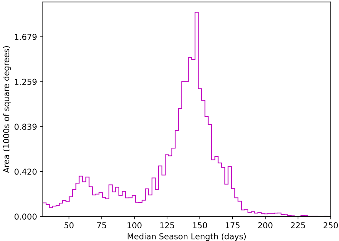
internal_u_expt45_nscale1.5v3.4_10yrs All sky z band: Median Season Length
