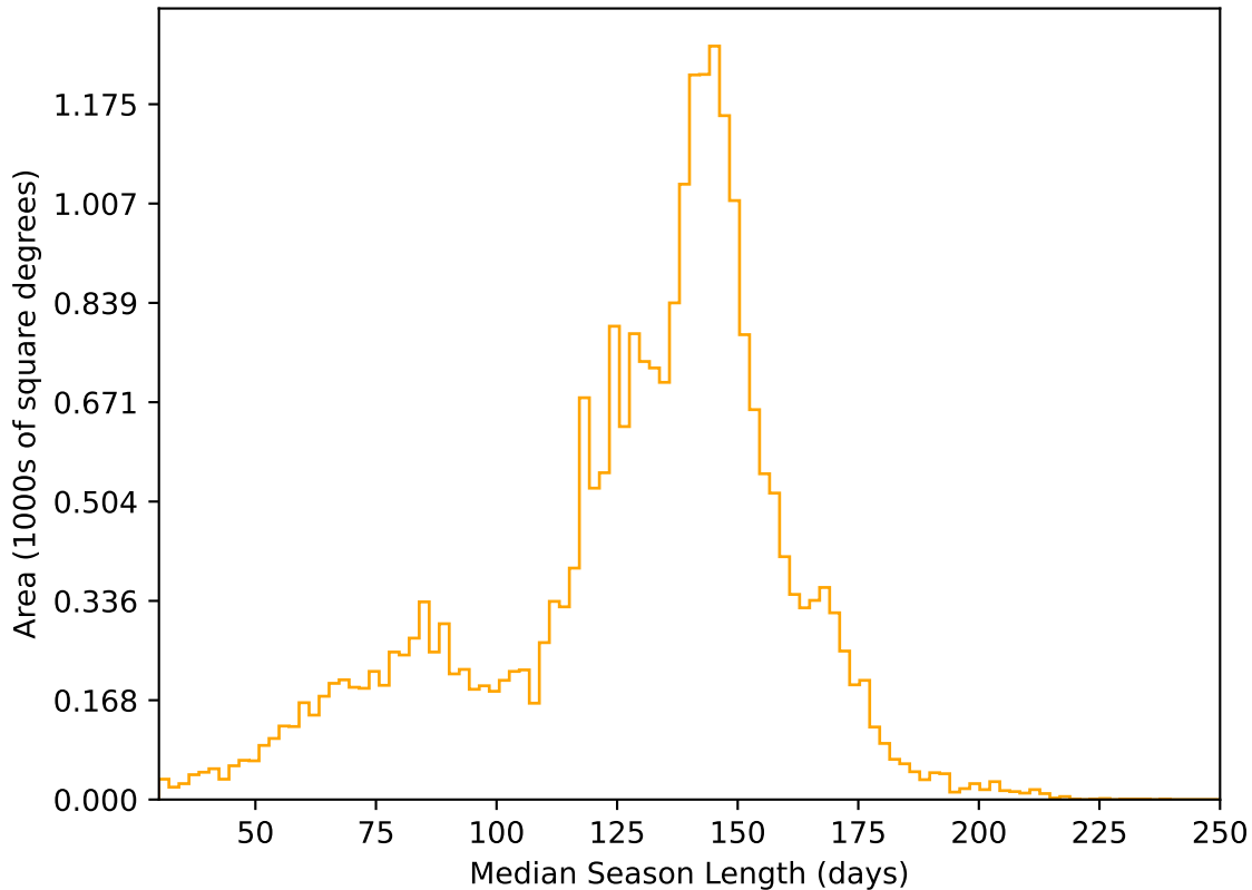
internal_u_expt45_nscale1.5v3.4_10yrs All sky r band: Median Season Length
