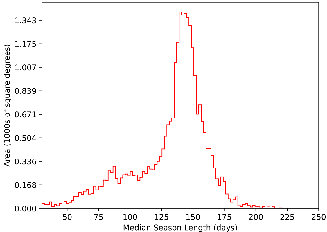
internal_u_expt45_nscale1.5v3.4_10yrs All sky i band: Median Season Length
