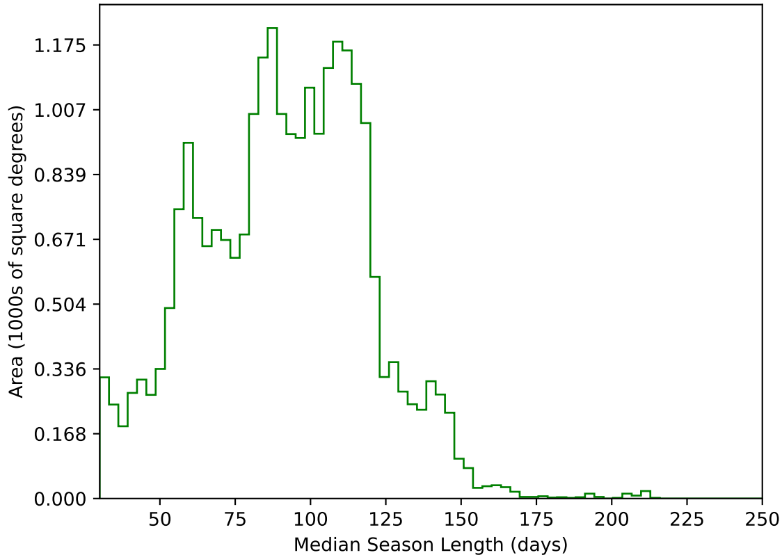
internal_u_expt45_nscale1.5v3.4_10yrs All sky g band: Median Season Length
