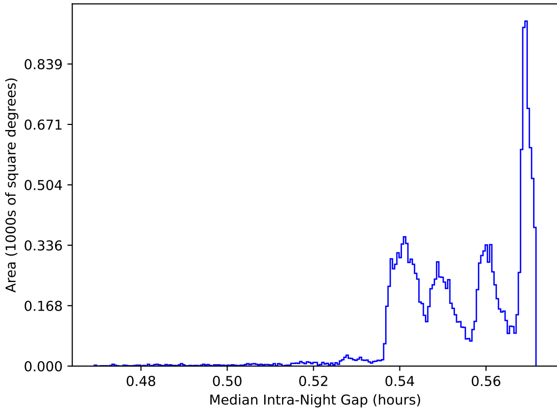
internal_u_expt45_nscale1.5v3.4_10yrs WFD: Median Intra-Night Gap
