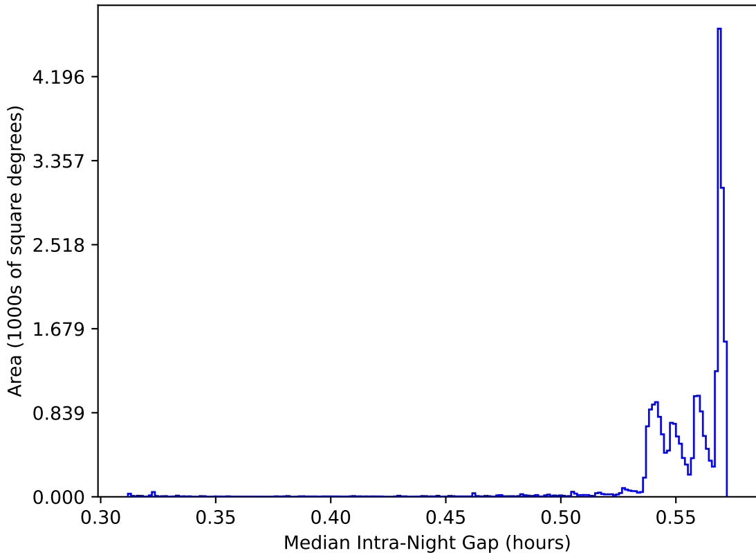
internal_u_expt45_nscale1.5v3.4_10yrs All sky: Median Intra-Night Gap
