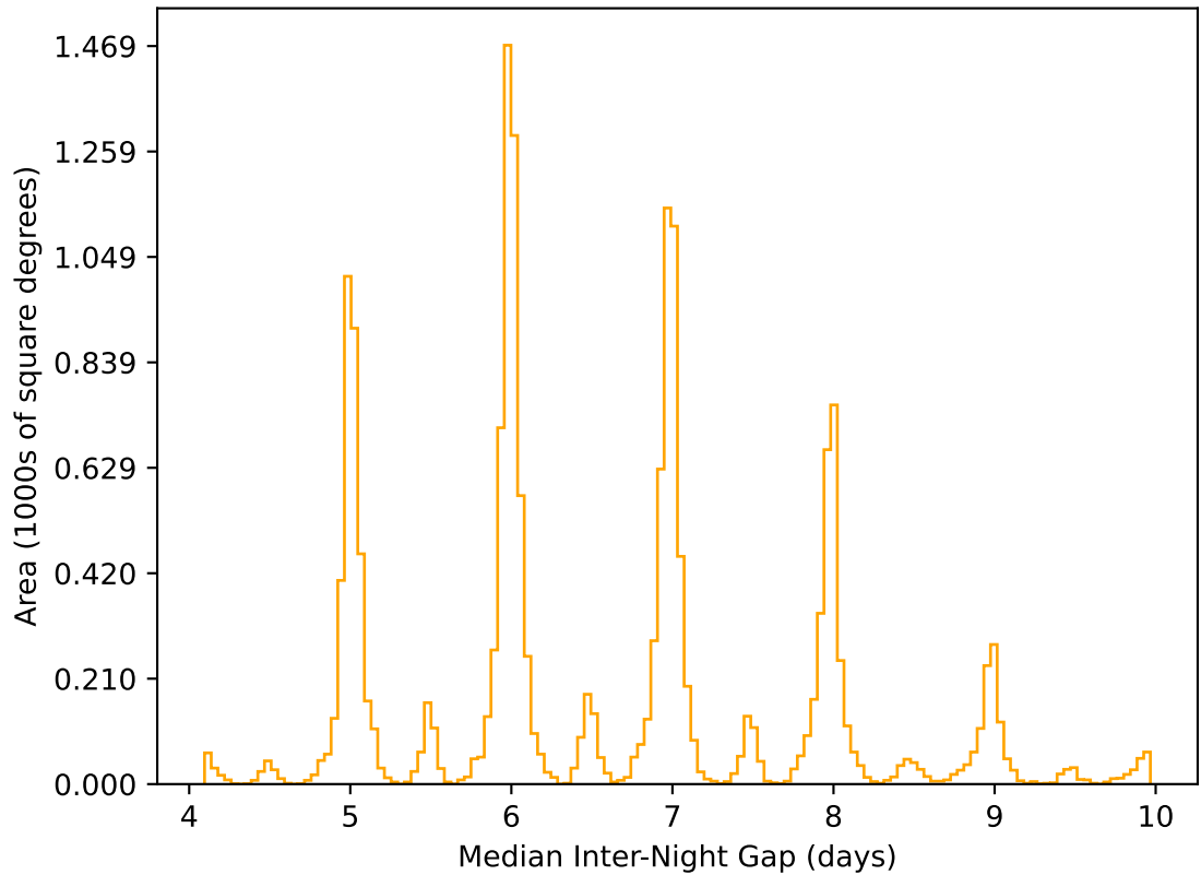
internal_u_expt45_nscale1.5v3.4_10yrs WFD r band: Median Inter-Night Gap
