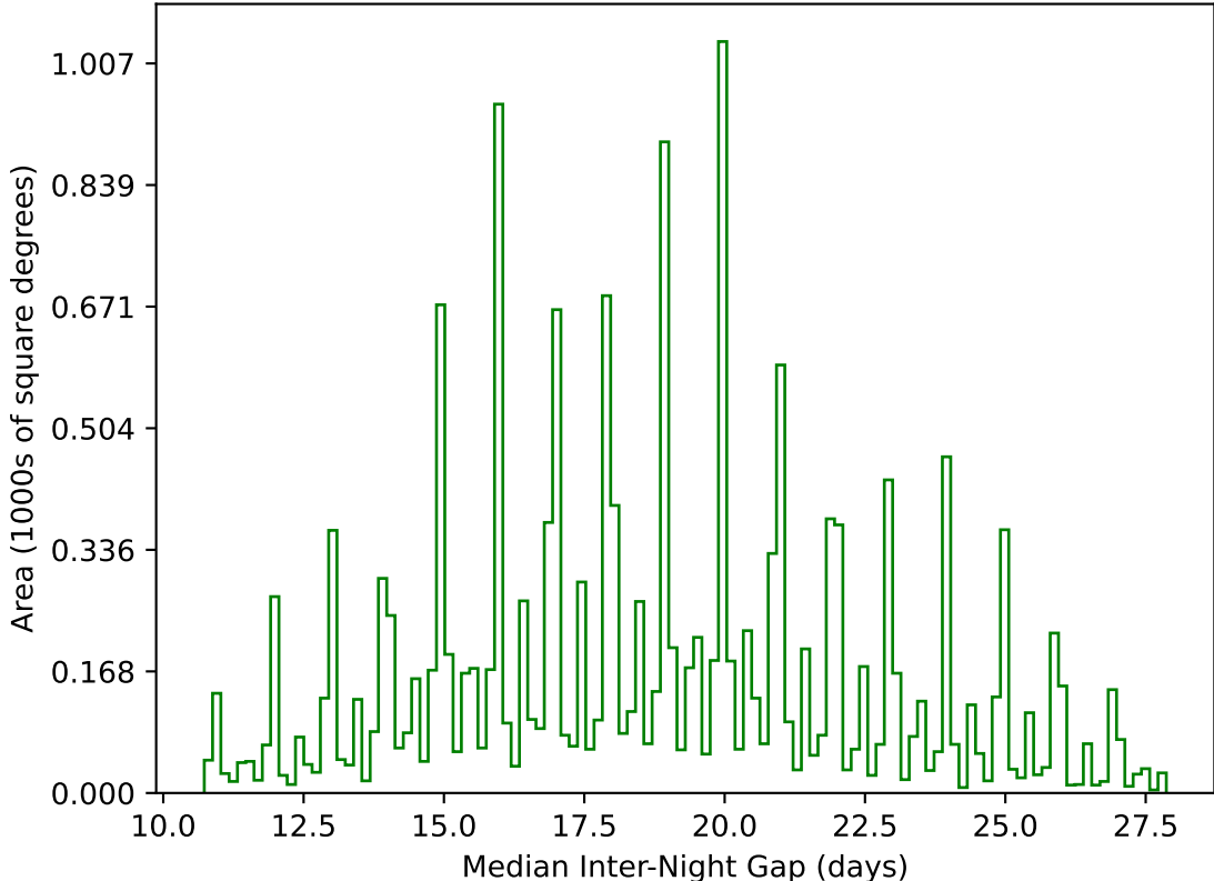
internal_u_expt45_nscale1.5v3.4_10yrs WFD g band: Median Inter-Night Gap
