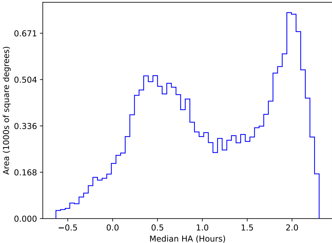
internal_u_expt45_nscale1.5v3.4_10yrs WFD z band: Median HA
