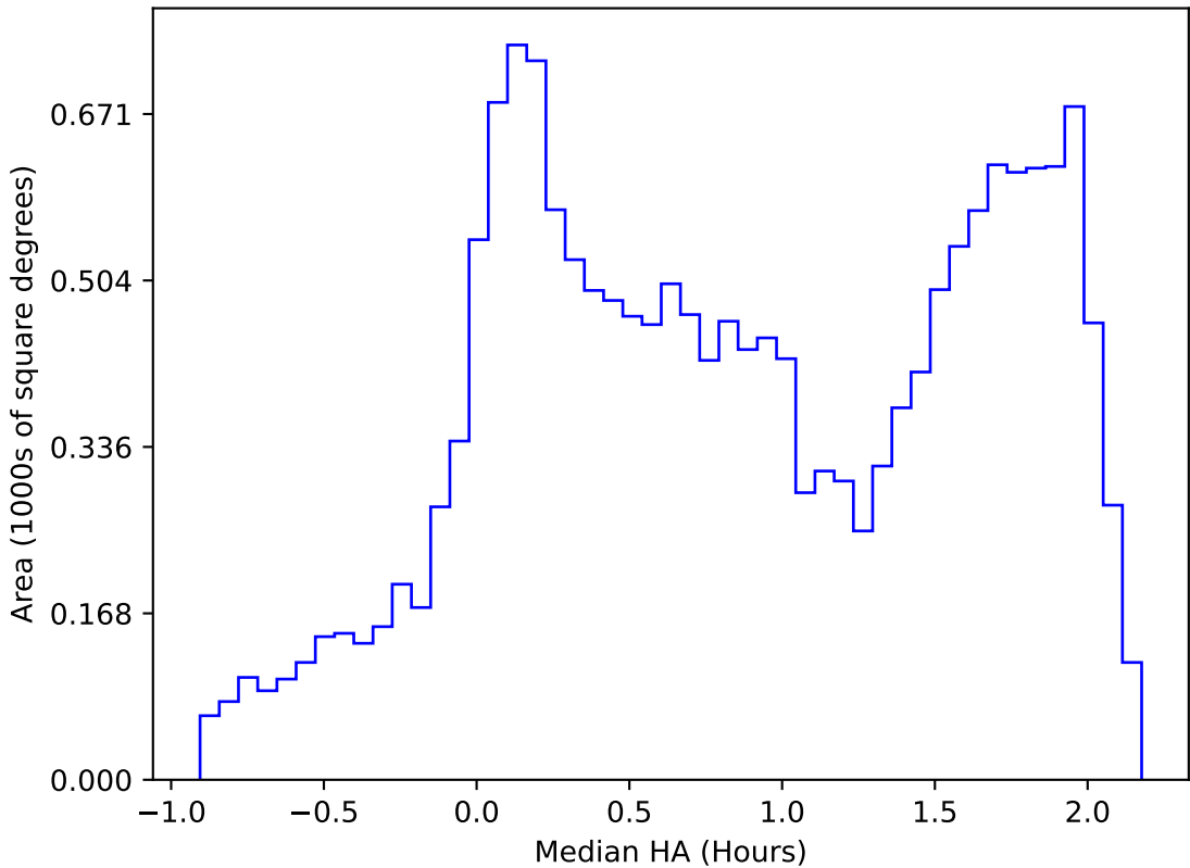
internal_u_expt45_nscale1.5v3.4_10yrs WFD r band: Median HA
