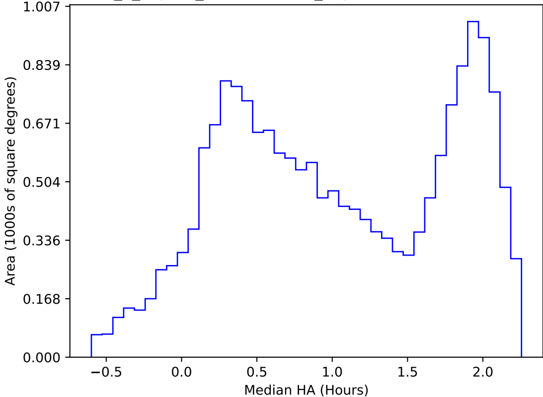
internal_u_expt45_nscale1.5v3.4_10yrs WFD i band: Median HA
