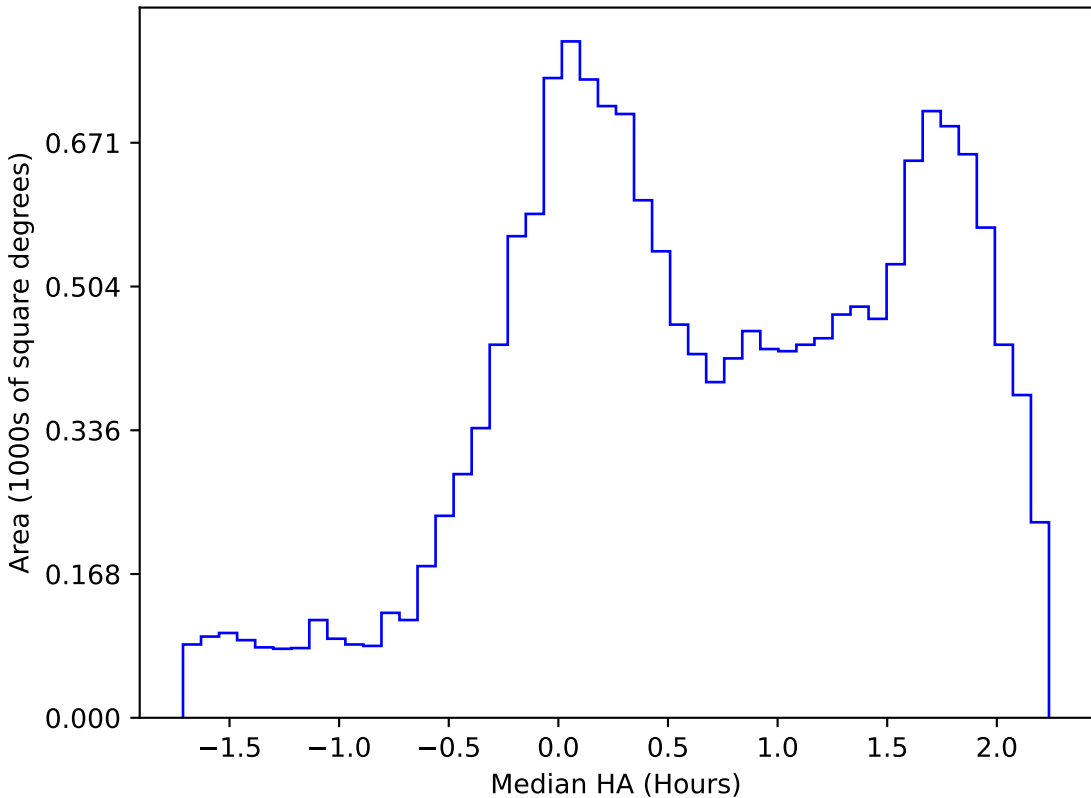
internal_u_expt45_nscale1.5v3.4_10yrs WFD g band: Median HA
