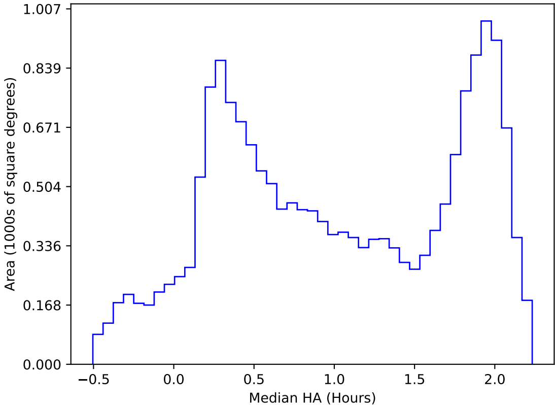
internal_u_expt45_nscale1.5v3.4_10yrs WFD all bands: Median HA
