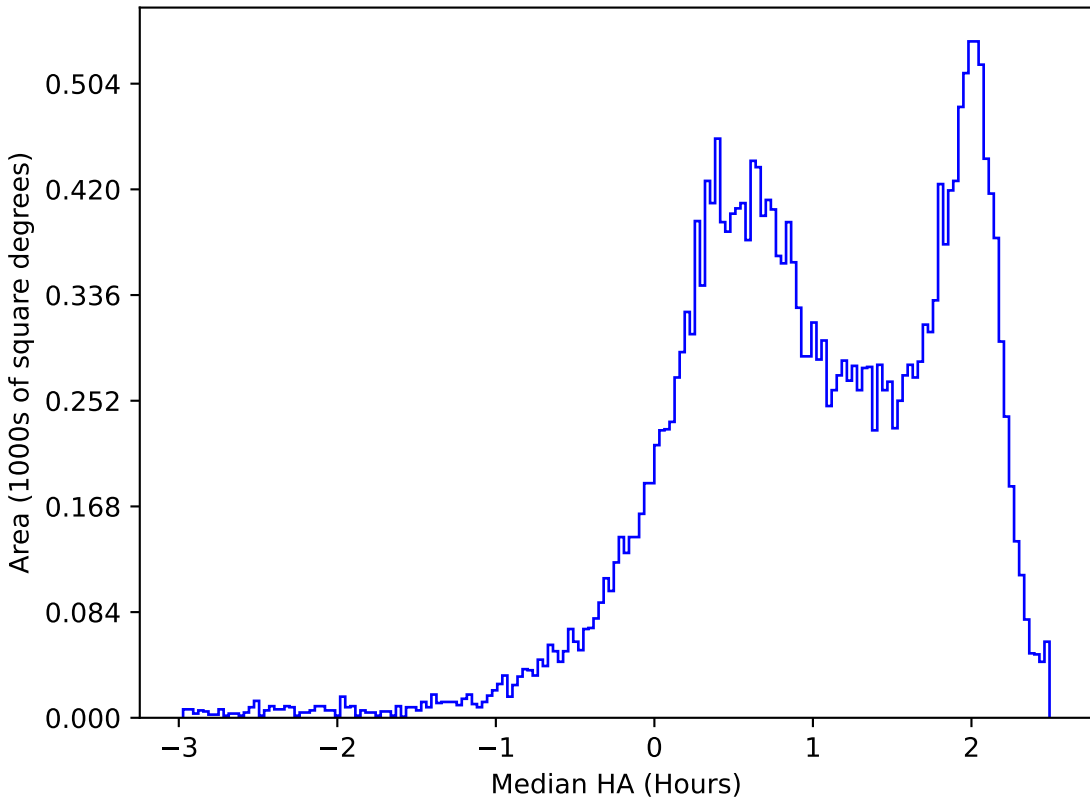
internal_u_expt45_nscale1.5v3.4_10yrs All sky z band: Median HA
