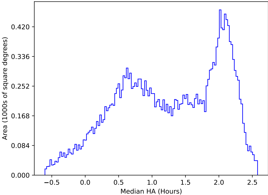
internal_u_expt45_nscale1.5v3.4_10yrs All sky y band: Median HA
