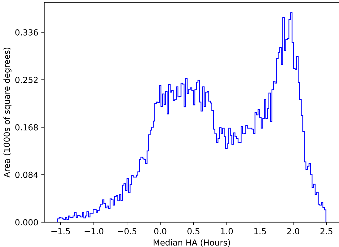
internal_u_expt45_nscale1.5v3.4_10yrs All sky u band: Median HA
