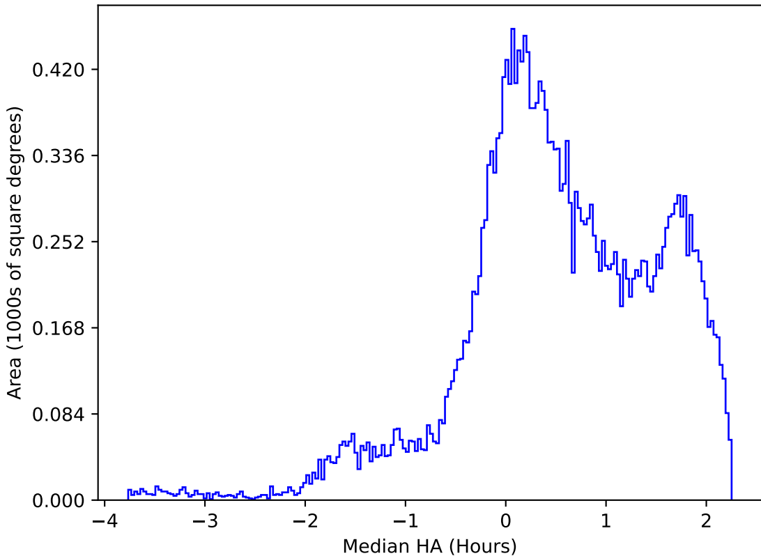
internal_u_expt45_nscale1.5v3.4_10yrs All sky g band: Median HA
