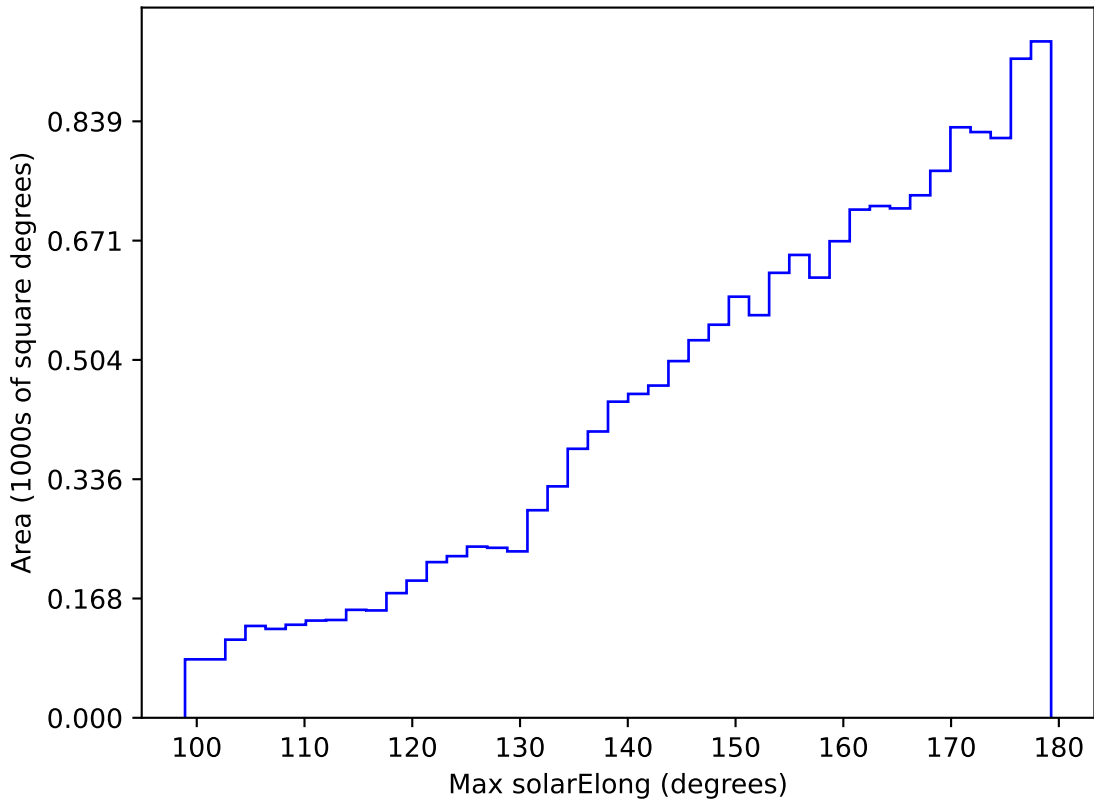
internal_u_expt45_nscale1.5v3.4_10yrs WFD y band: Max solarElong
