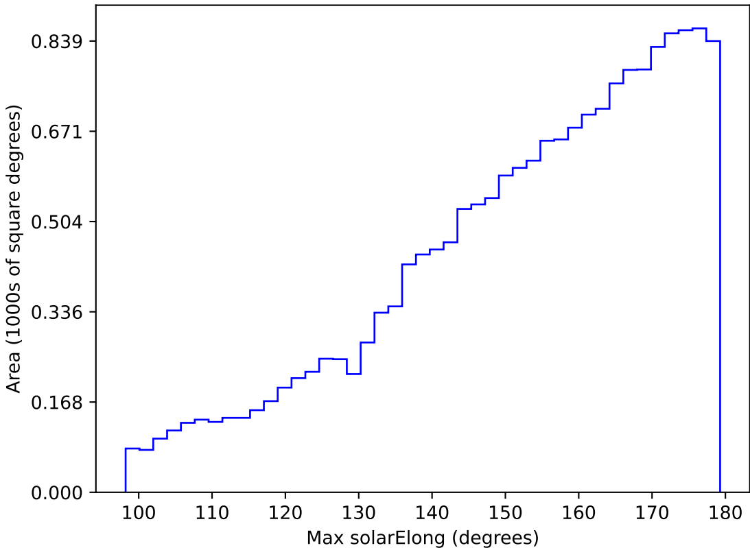
internal_u_expt45_nscale1.5v3.4_10yrs WFD u band: Max solarElong
