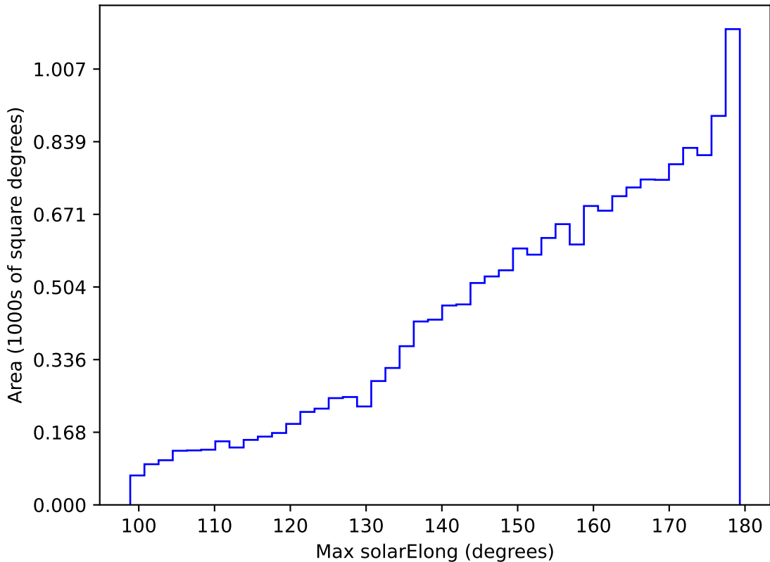
internal_u_expt45_nscale1.5v3.4_10yrs WFD i band: Max solarElong
