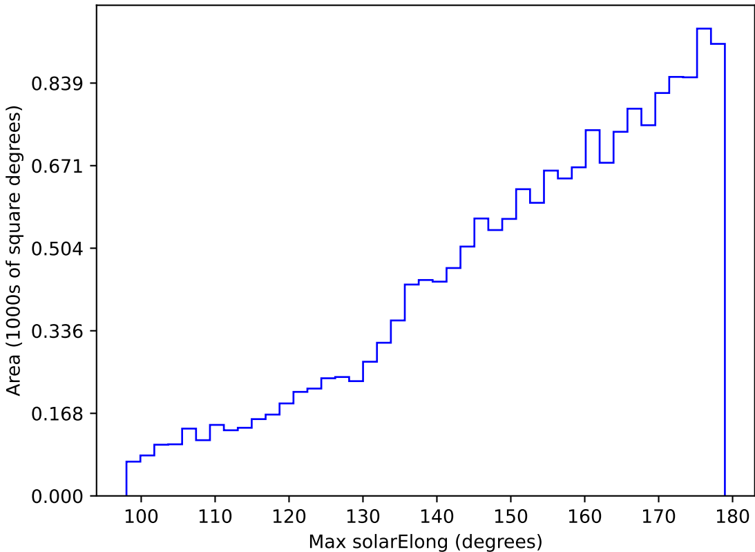
internal_u_expt45_nscale1.5v3.4_10yrs WFD g band: Max solarElong
