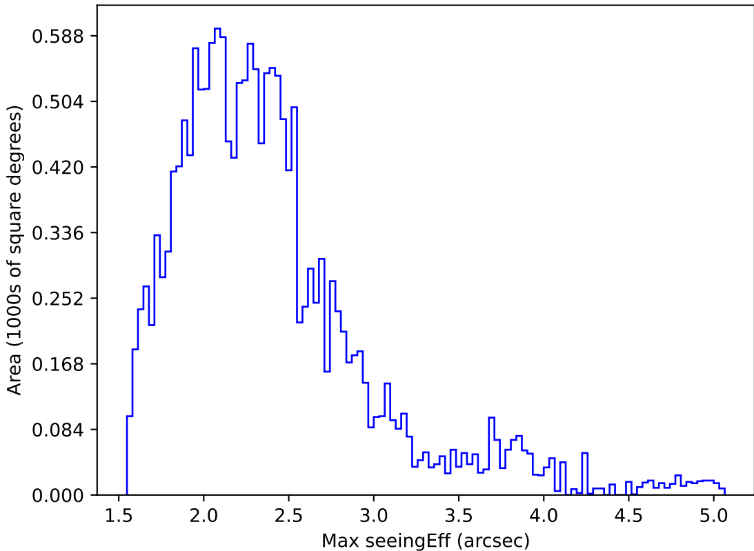
internal_u_expt45_nscale1.5v3.4_10yrs WFD y band: Max seeingEff
