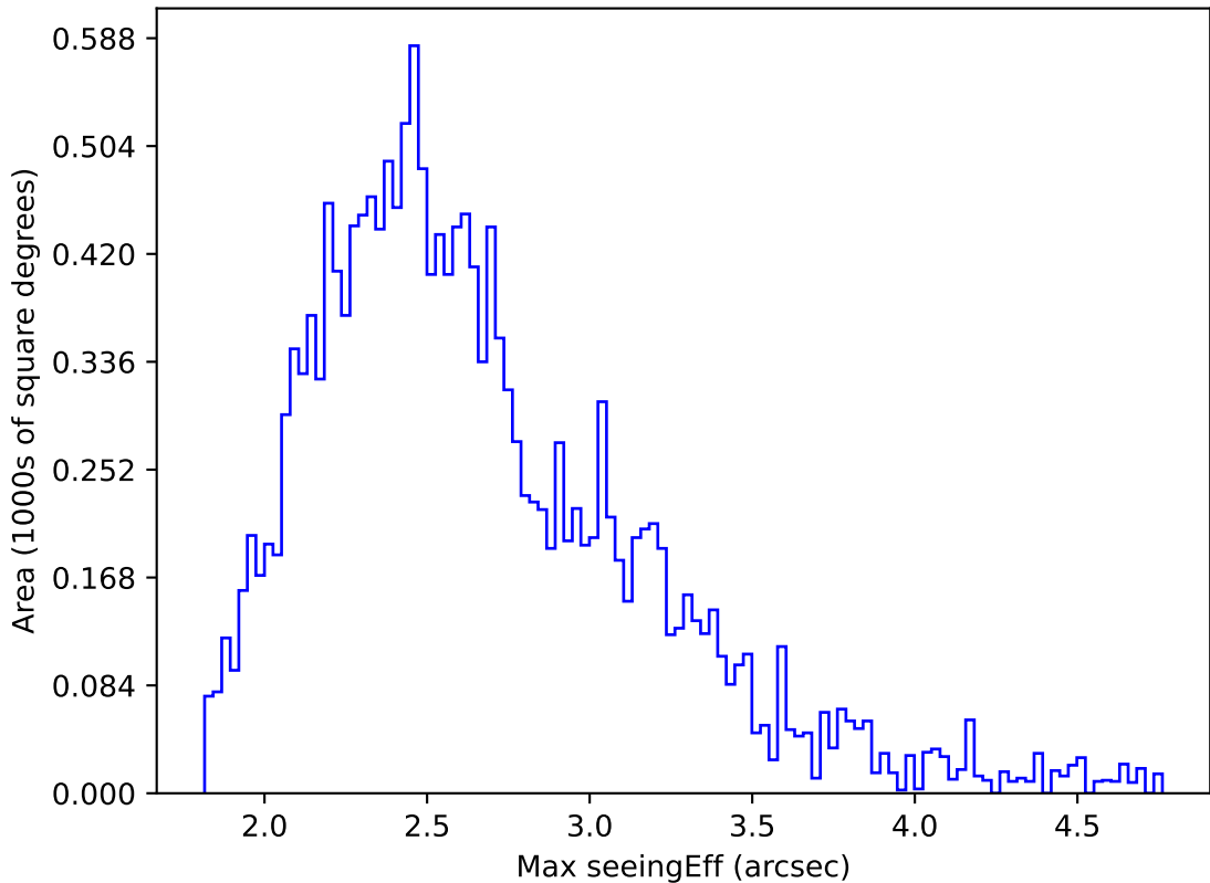
internal_u_expt45_nscale1.5v3.4_10yrs WFD u band: Max seeingEff
