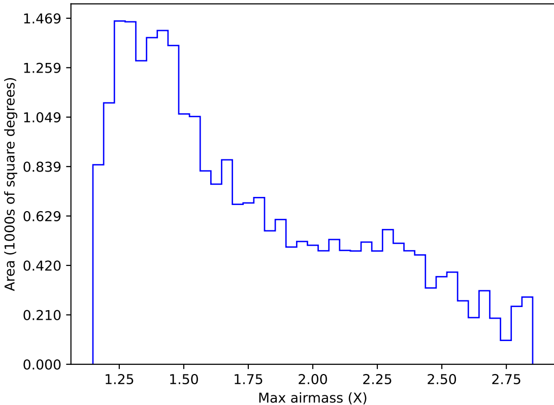
internal_u_expt45_nscale1.5v3.4_10yrs Yr 1 z band: Max airmass
