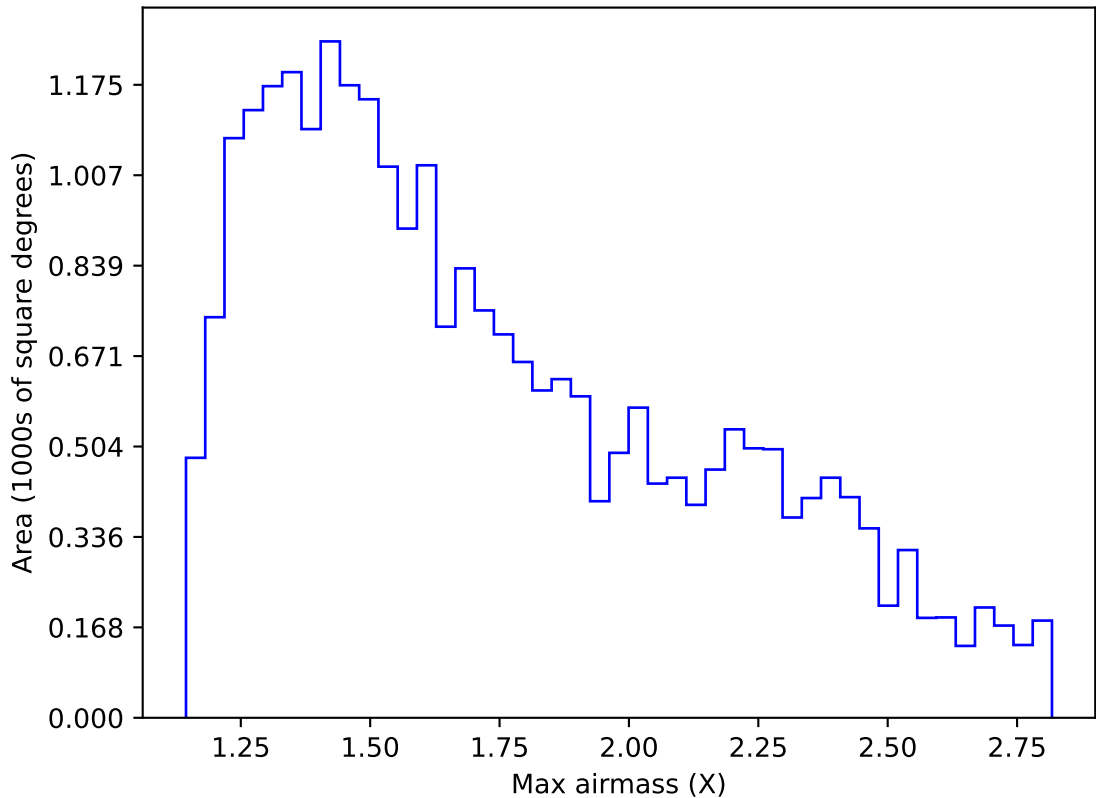
internal_u_expt45_nscale1.5v3.4_10yrs Yr 1 i band: Max airmass
