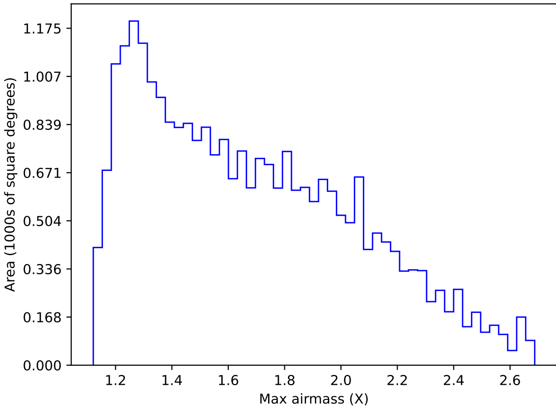
internal_u_expt45_nscale1.5v3.4_10yrs Yr 1 g band: Max airmass
