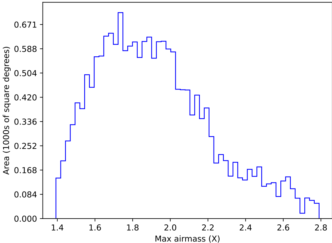
internal_u_expt45_nscale1.5v3.4_10yrs WFD u band: Max airmass
