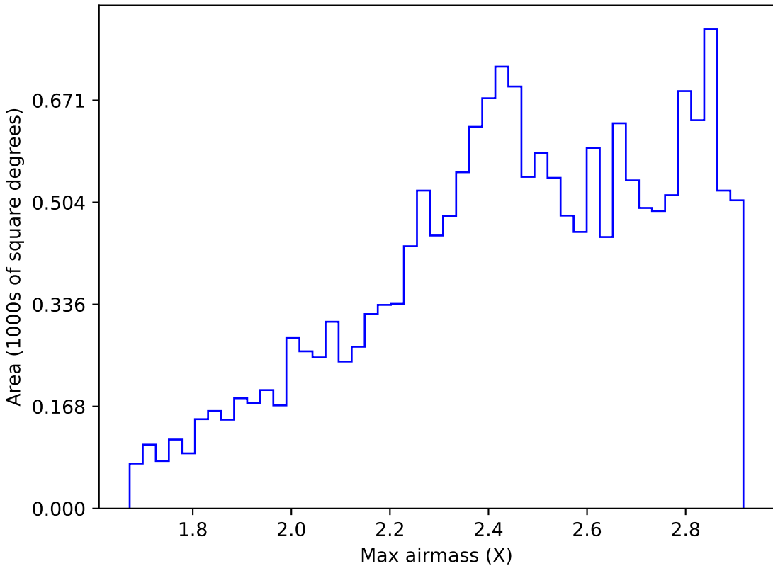
internal_u_expt45_nscale1.5v3.4_10yrs WFD i band: Max airmass
