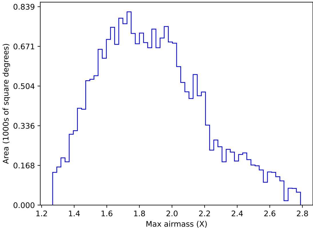
internal_u_expt45_nscale1.5v3.4_10yrs All sky u band: Max airmass
