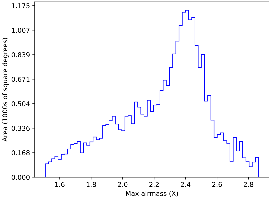
internal_u_expt45_nscale1.5v3.4_10yrs All sky r band: Max airmass
