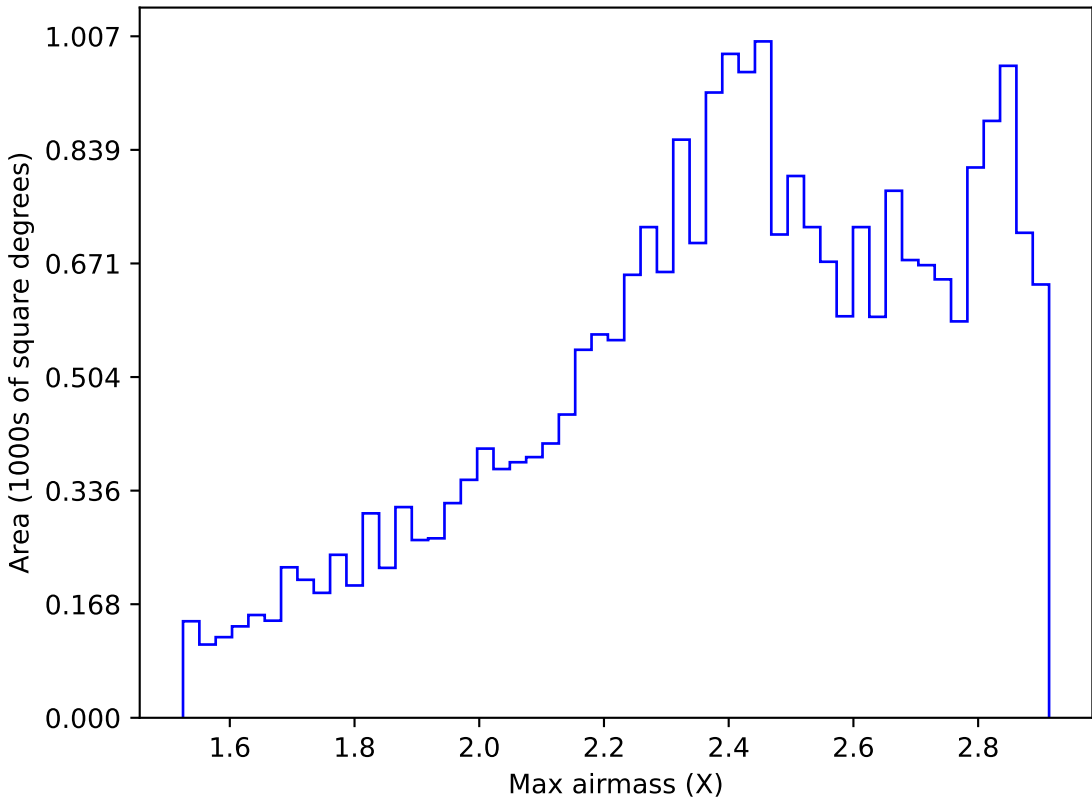
internal_u_expt45_nscale1.5v3.4_10yrs All sky i band: Max airmass
