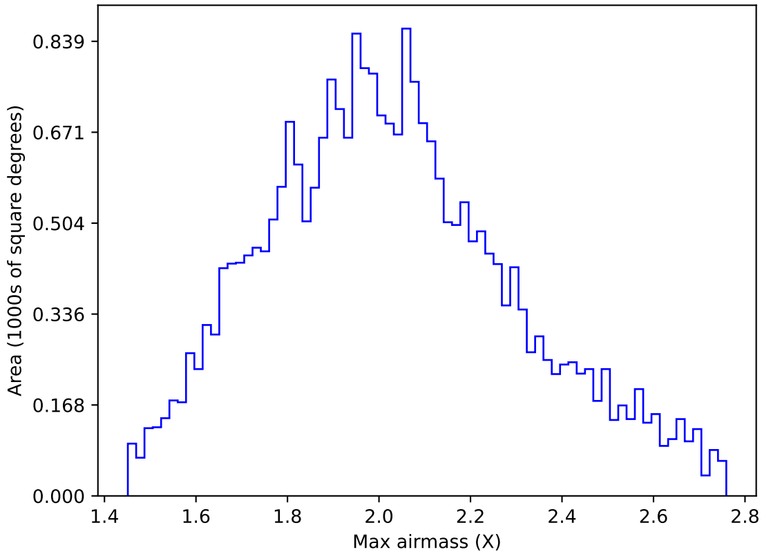
internal_u_expt45_nscale1.5v3.4_10yrs All sky g band: Max airmass
