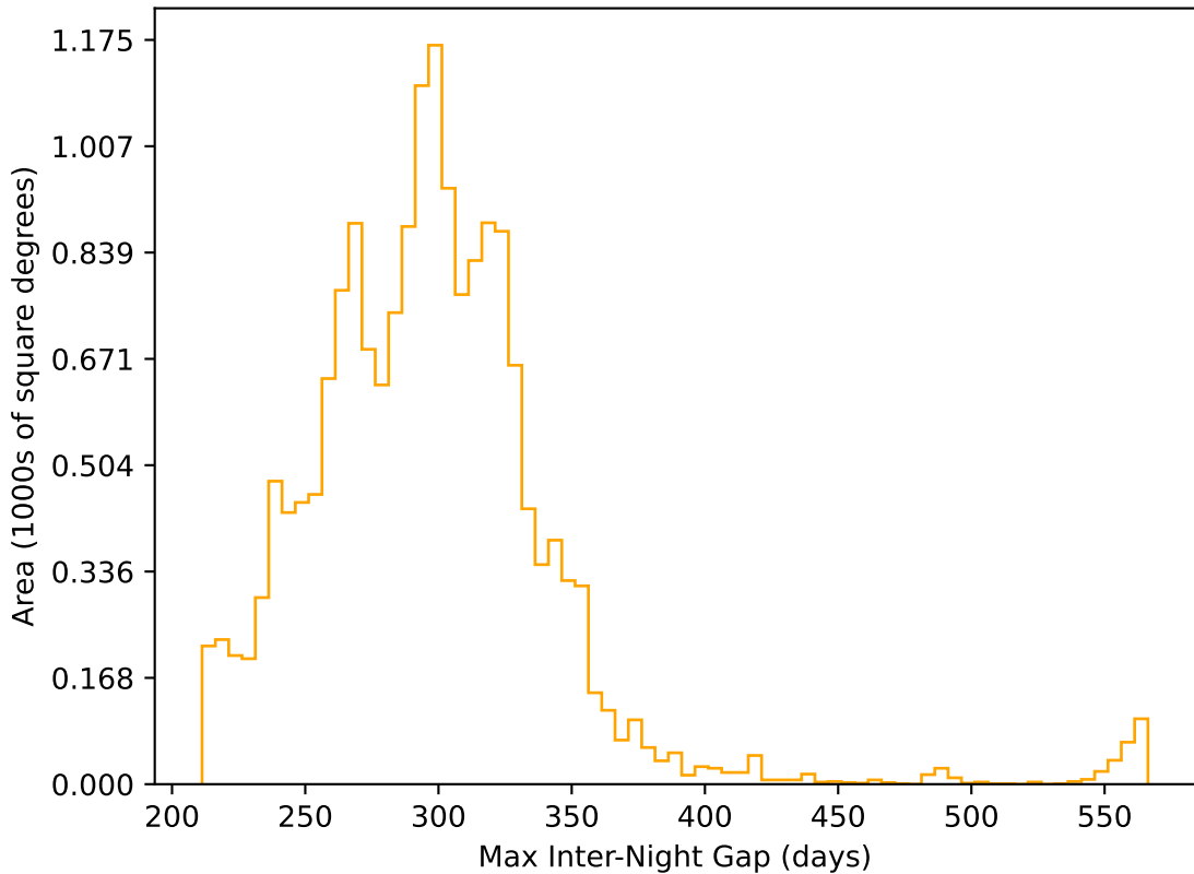
internal_u_expt45_nscale1.5v3.4_10yrs WFD r band: Max Inter-Night Gap
