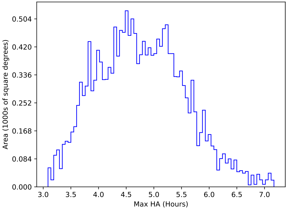
internal_u_expt45_nscale1.5v3.4_10yrs WFD i band: Max HA
