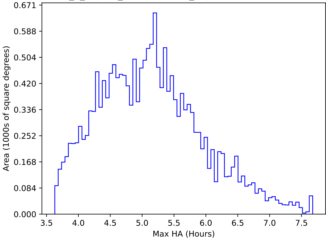
internal_u_expt45_nscale1.5v3.4_10yrs WFD all bands: Max HA
