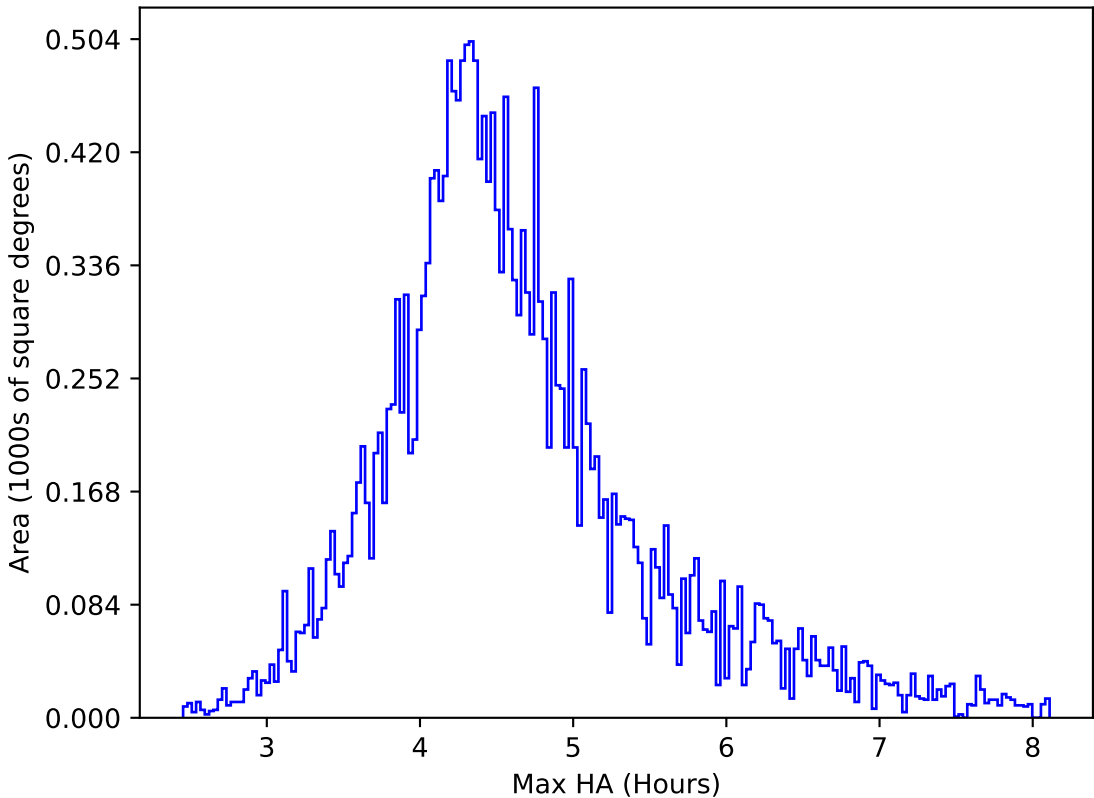
internal_u_expt45_nscale1.5v3.4_10yrs All sky y band: Max HA
