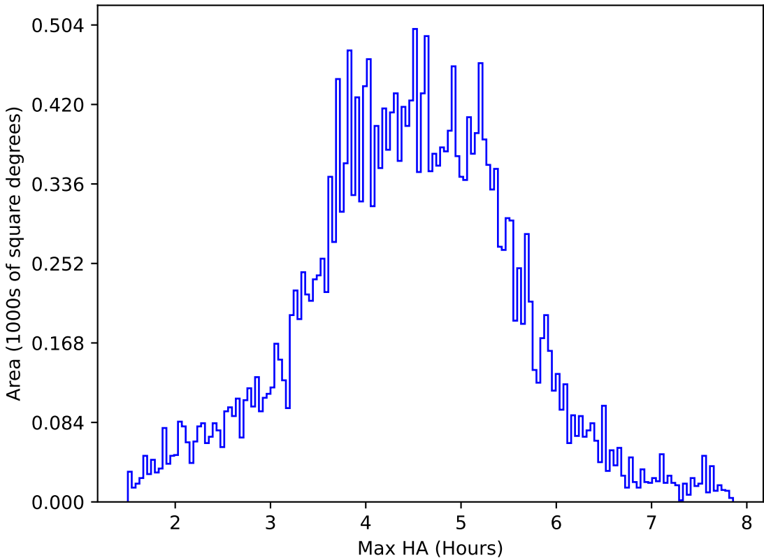
internal_u_expt45_nscale1.5v3.4_10yrs All sky i band: Max HA
