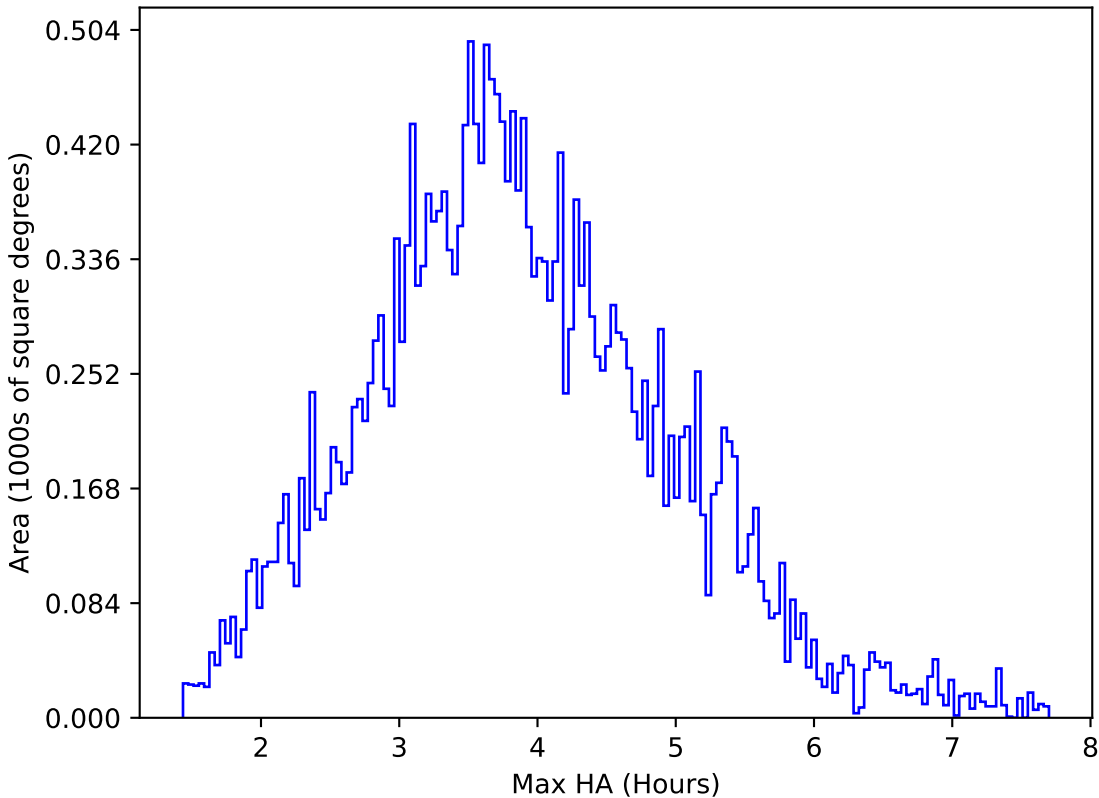
internal_u_expt45_nscale1.5v3.4_10yrs All sky g band: Max HA
