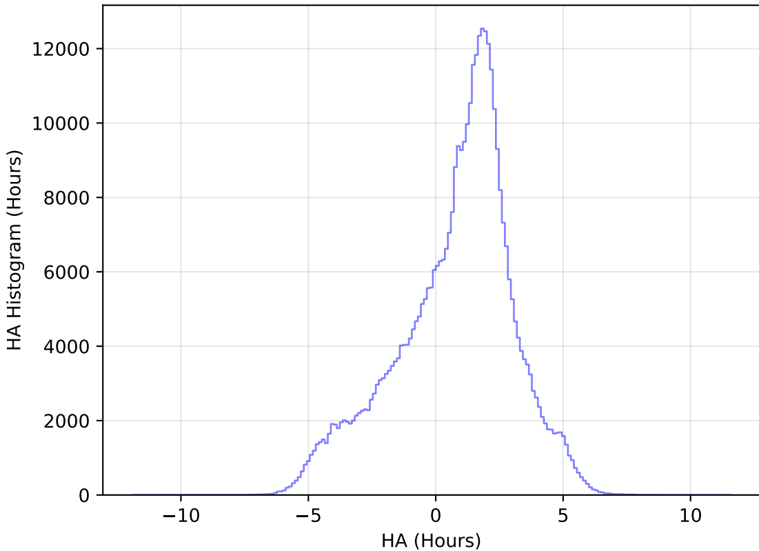
internal_u_expt45_nscale1.5v3.4_10yrs WFD z band: HA Histogram
