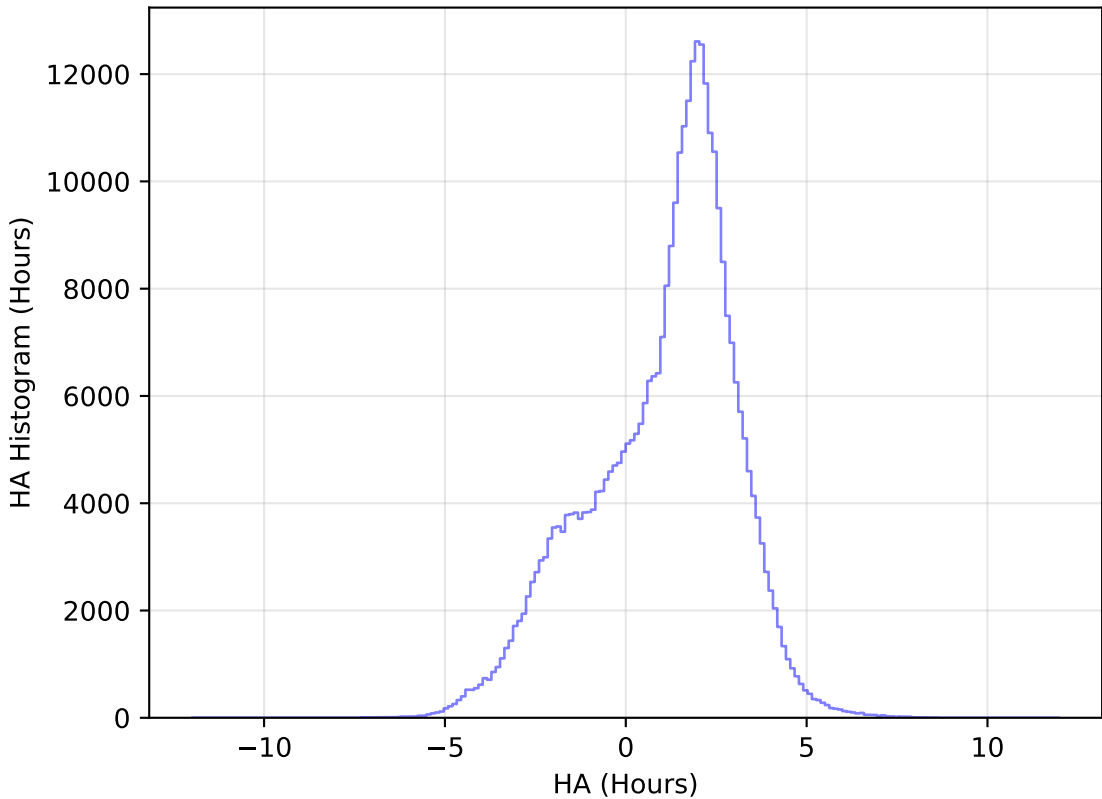
internal_u_expt45_nscale1.5v3.4_10yrs WFD y band: HA Histogram
