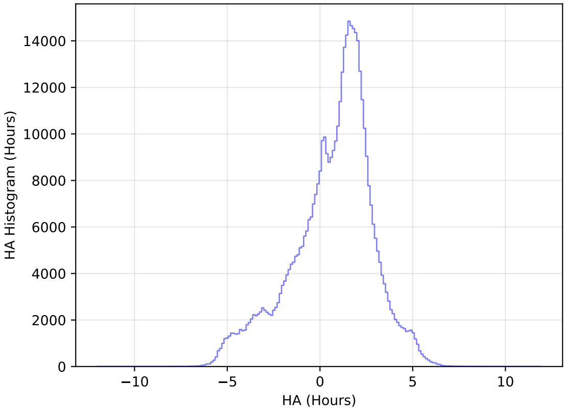
internal_u_expt45_nscale1.5v3.4_10yrs WFD i band: HA Histogram
