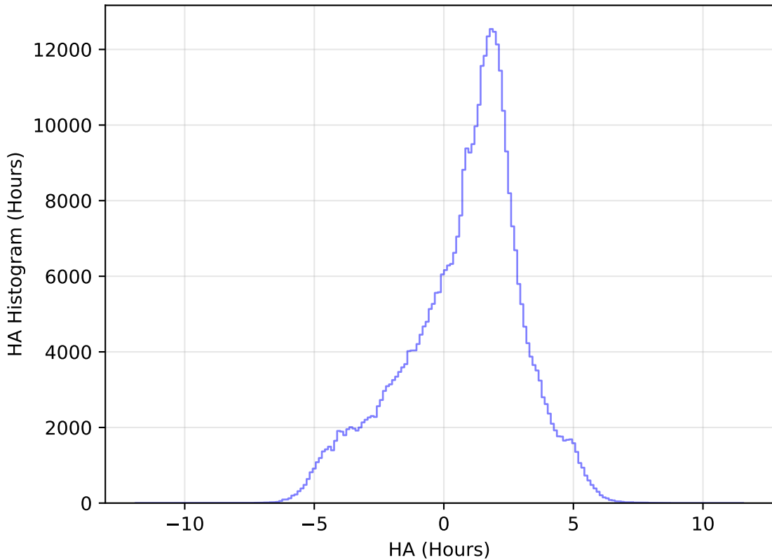
internal_u_expt45_nscale1.5v3.4_10yrs All sky z band: HA Histogram
