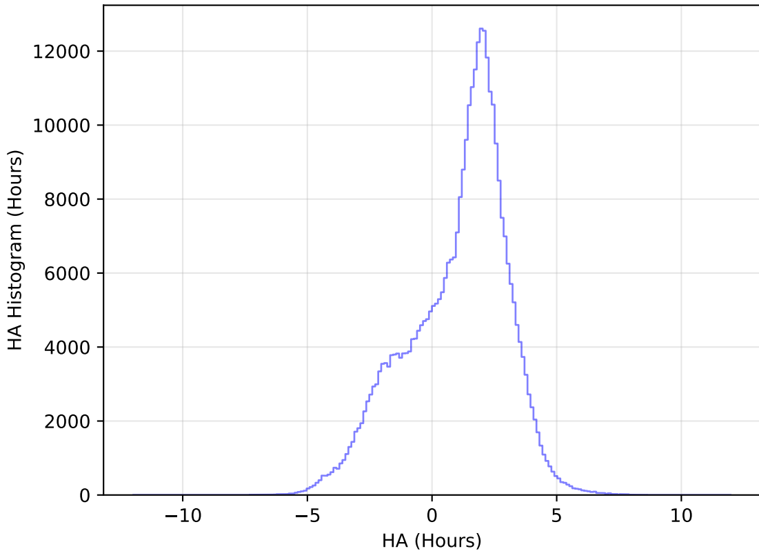
internal_u_expt45_nscale1.5v3.4_10yrs All sky y band: HA Histogram
