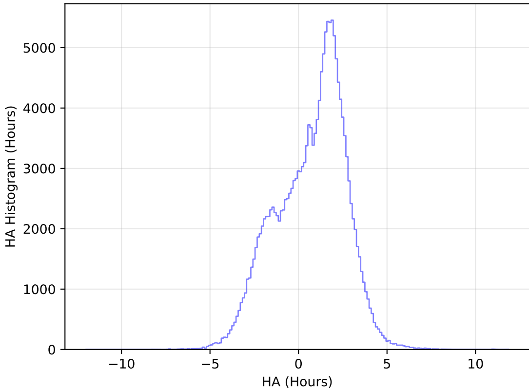
internal_u_expt45_nscale1.5v3.4_10yrs All sky u band: HA Histogram
